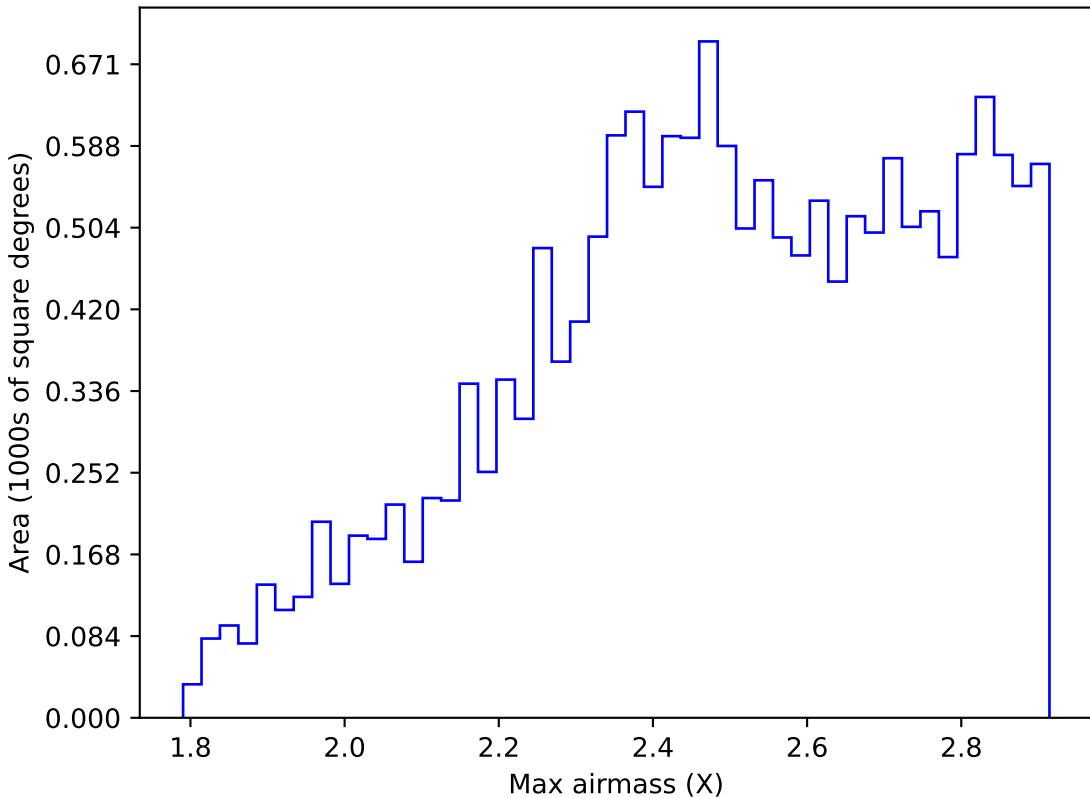
too_elab_r8_d2_griz_v3.4_10yrs WFD z band: Max airmass
