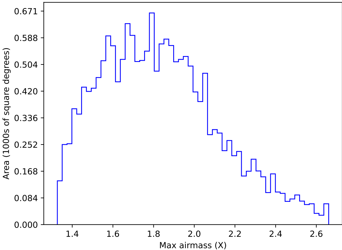
too_elab_r8_d2_griz_v3.4_10yrs WFD u band: Max airmass
