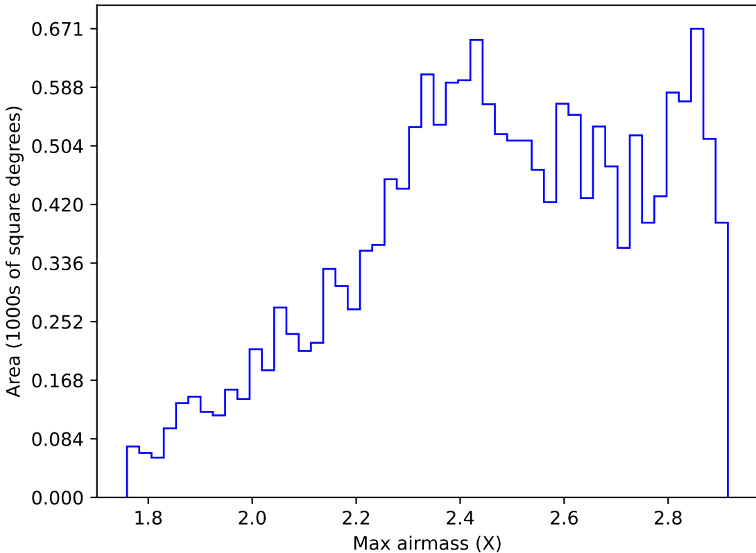
too_elab_r8_d2_griz_v3.4_10yrs WFD i band: Max airmass
