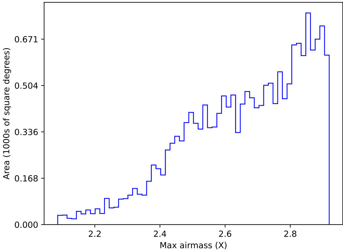
too_elab_r8_d2_griz_v3.4_10yrs WFD all bands: Max airmass
