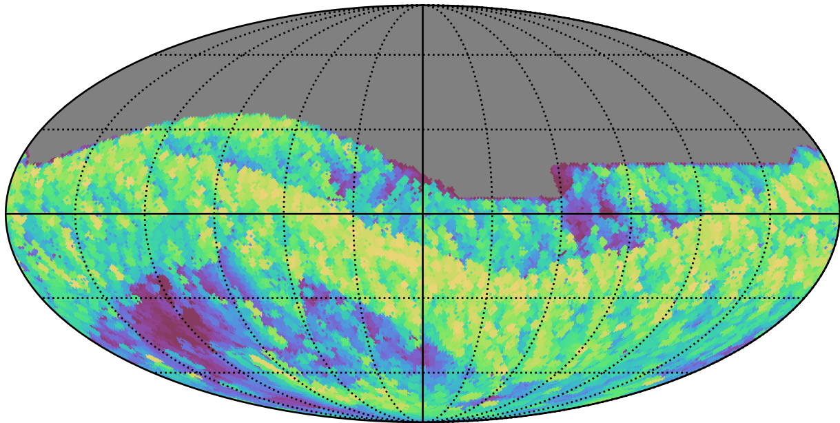
too_elab_r8_d2_griz_v3.4_10yrs All sky z band: Max airmass
