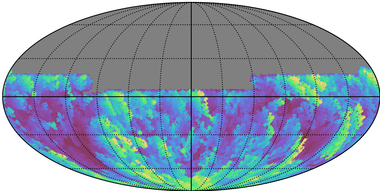
too_elab_r8_d2_griz_v3.4_10yrs All sky u band: Max airmass
