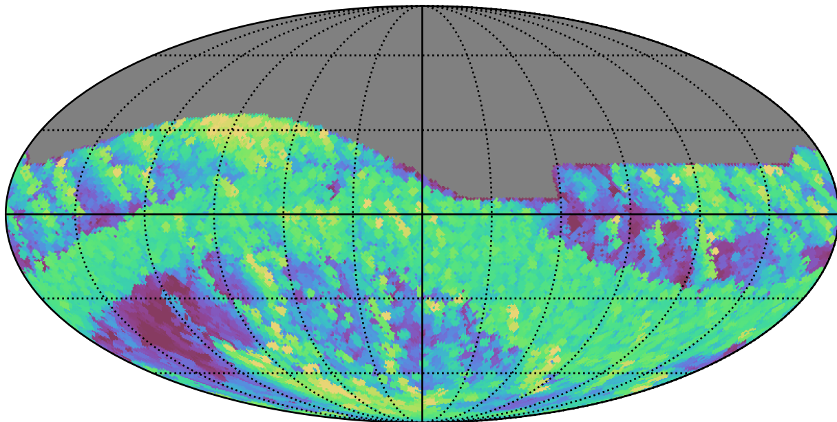
too_elab_r8_d2_griz_v3.4_10yrs All sky r band: Max airmass
