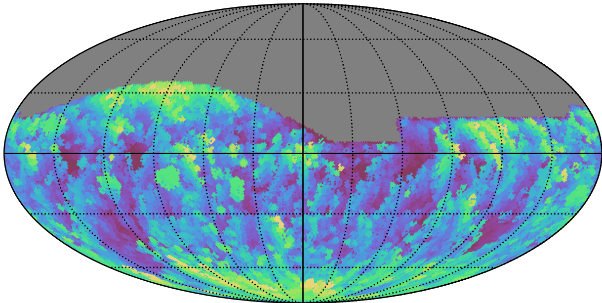
too_elab_r8_d2_griz_v3.4_10yrs All sky g band: Max airmass
