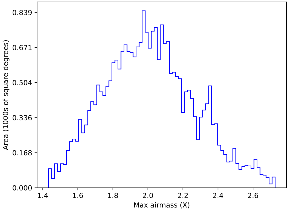
too_elab_r8_d2_griz_v3.4_10yrs All sky g band: Max airmass
