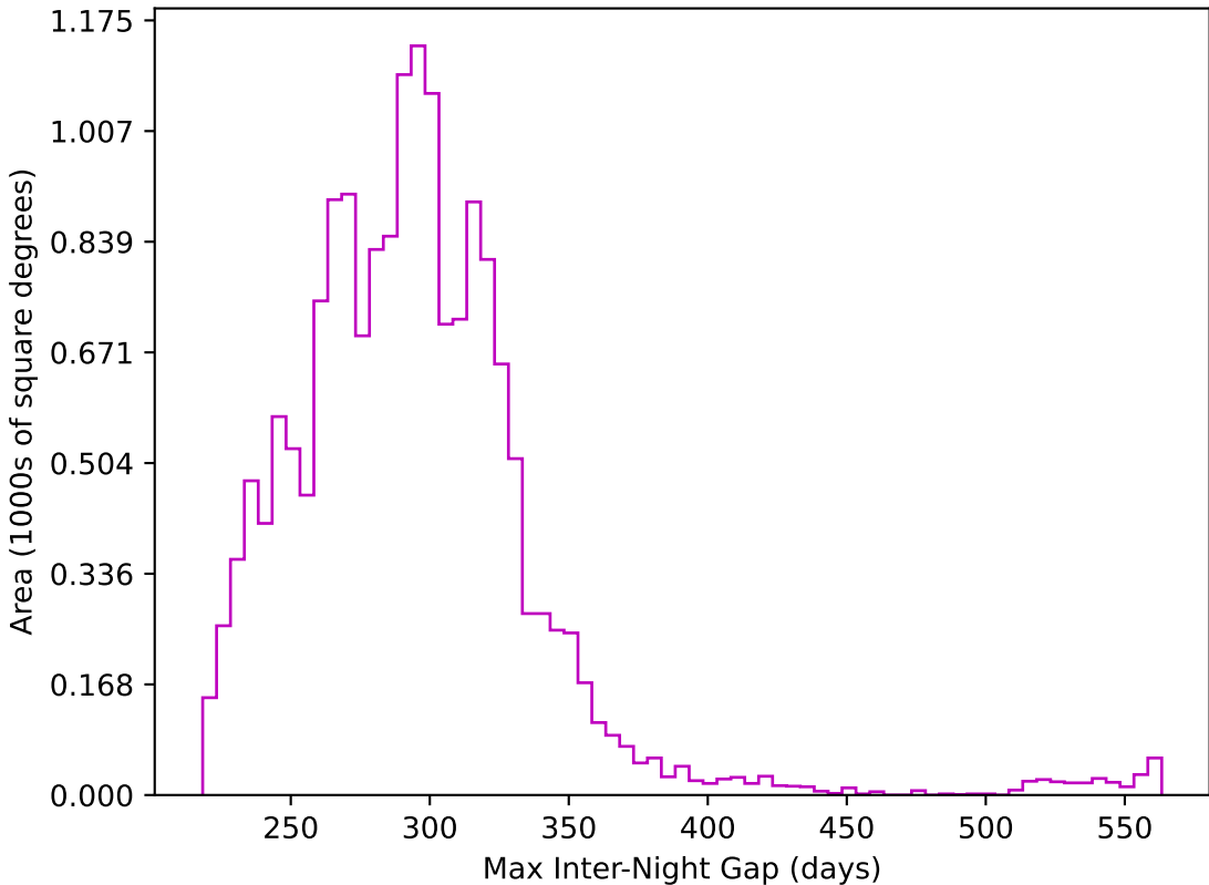
too_elab_r8_d2_griz_v3.4_10yrs WFD z band: Max Inter-Night Gap
