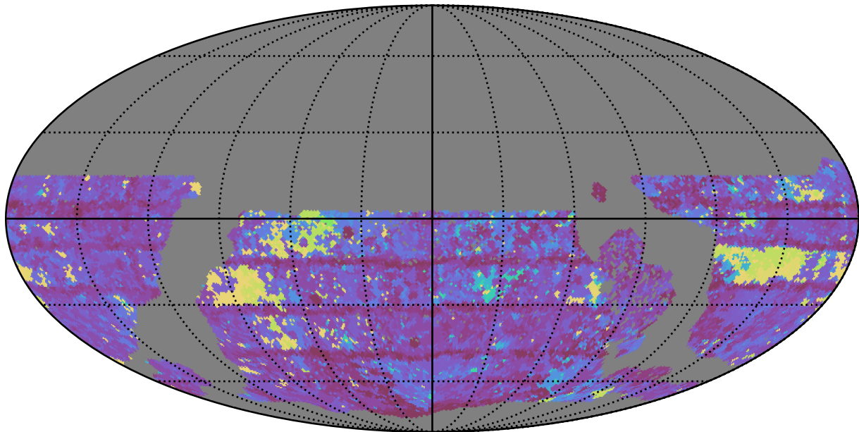
too_elab_r8_d2_griz_v3.4_10yrs WFD y band: Max Inter-Night Gap
