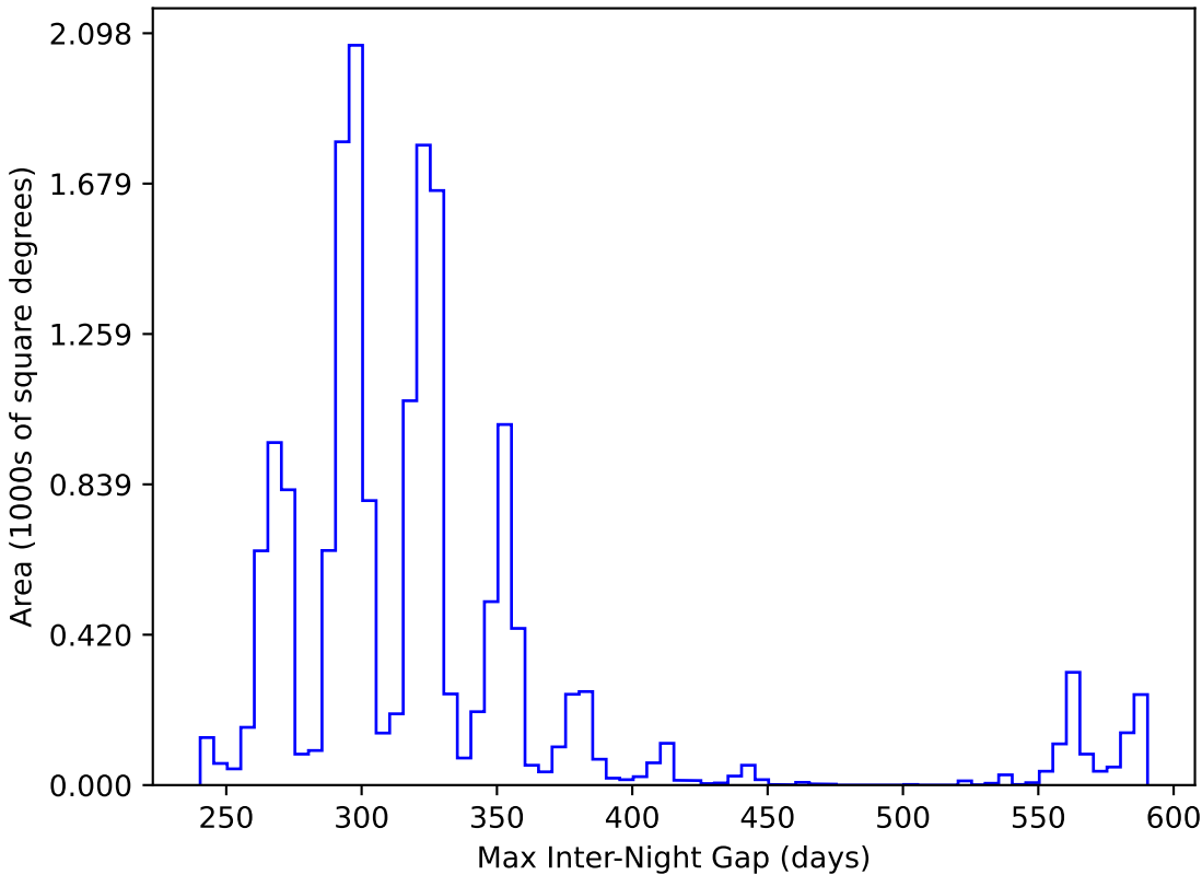
too_elab_r8_d2_griz_v3.4_10yrs WFD y band: Max Inter-Night Gap
