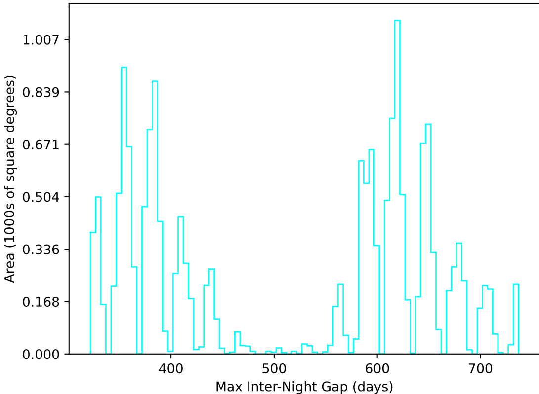
too_elab_r8_d2_griz_v3.4_10yrs WFD u band: Max Inter-Night Gap
