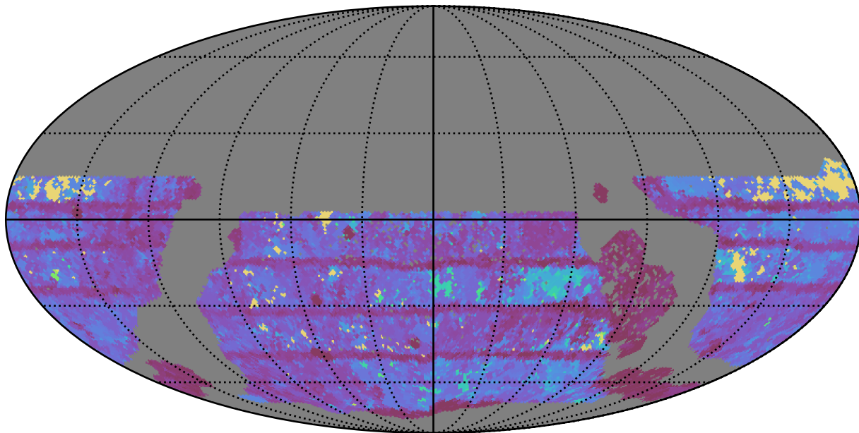
too_elab_r8_d2_griz_v3.4_10yrs WFD r band: Max Inter-Night Gap
