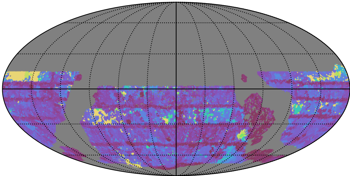
too_elab_r8_d2_griz_v3.4_10yrs WFD i band: Max Inter-Night Gap
