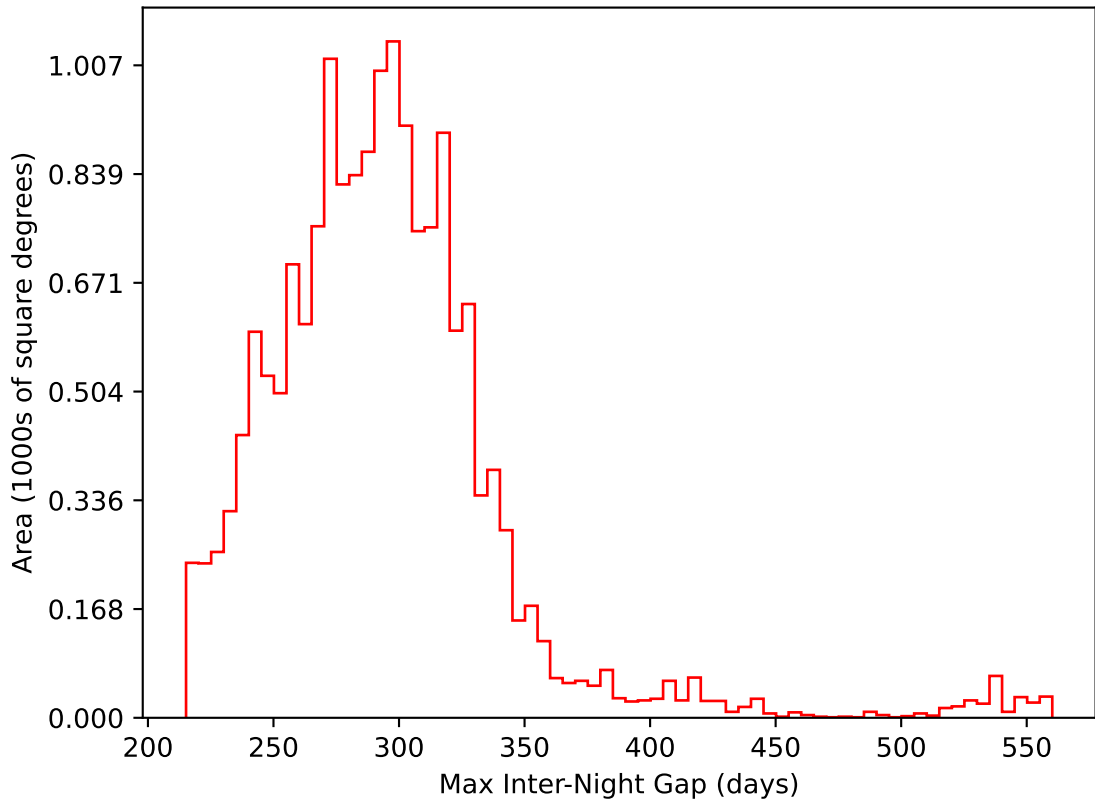
too_elab_r8_d2_griz_v3.4_10yrs WFD i band: Max Inter-Night Gap
