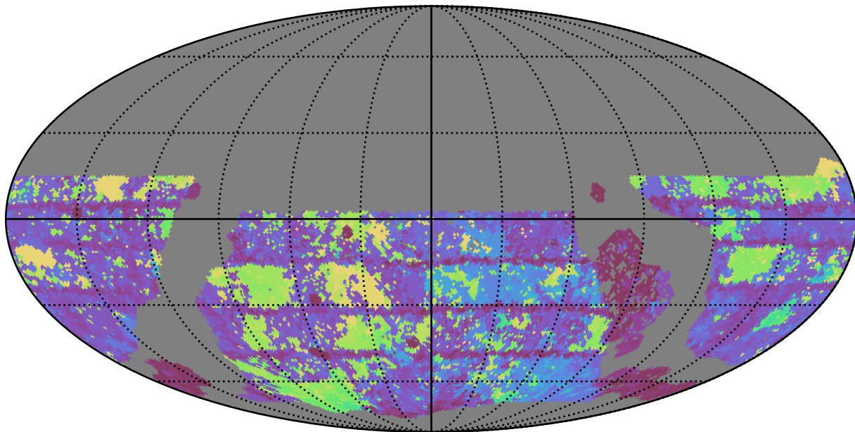
too_elab_r8_d2_griz_v3.4_10yrs WFD g band: Max Inter-Night Gap
