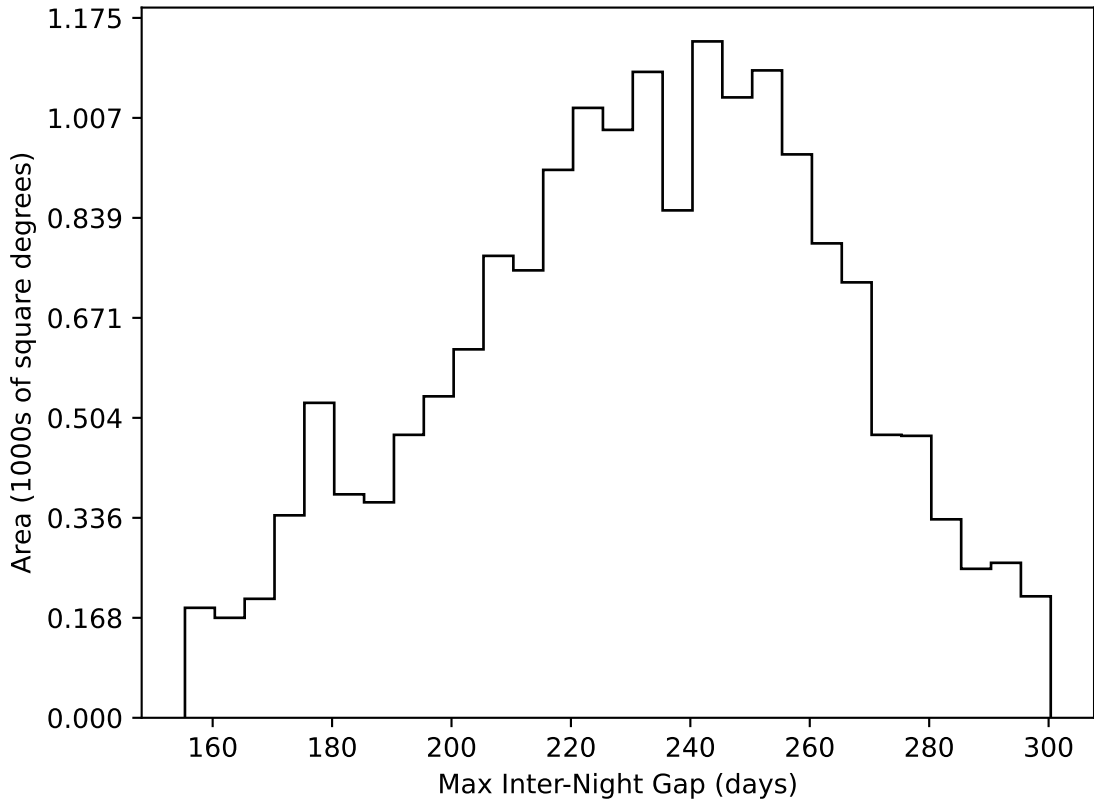
too_elab_r8_d2_griz_v3.4_10yrs WFD all bands: Max Inter-Night Gap
