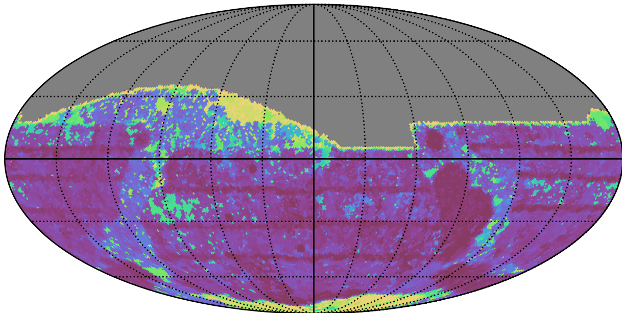
too_elab_r8_d2_griz_v3.4_10yrs All sky z band: Max Inter-Night Gap
