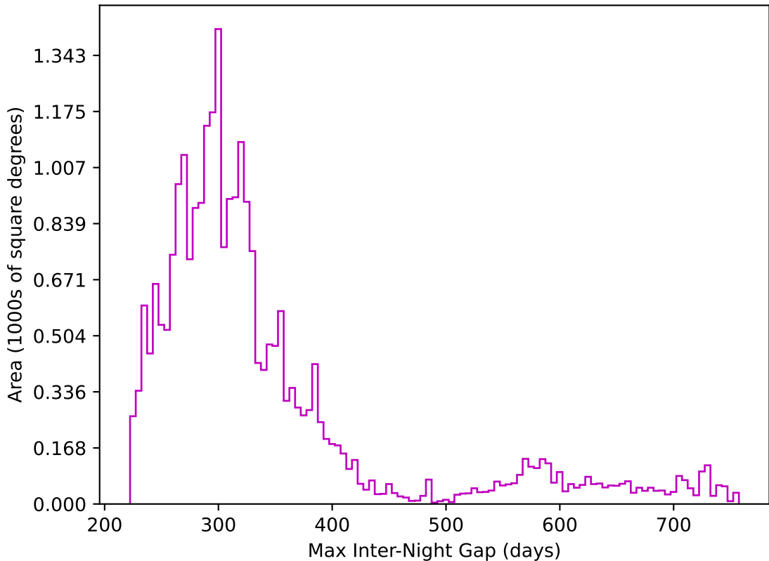
too_elab_r8_d2_griz_v3.4_10yrs All sky z band: Max Inter-Night Gap
