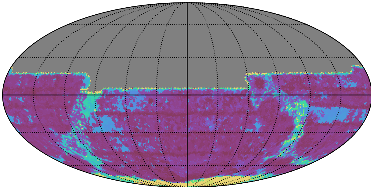
too_elab_r8_d2_griz_v3.4_10yrs All sky y band: Max Inter-Night Gap
