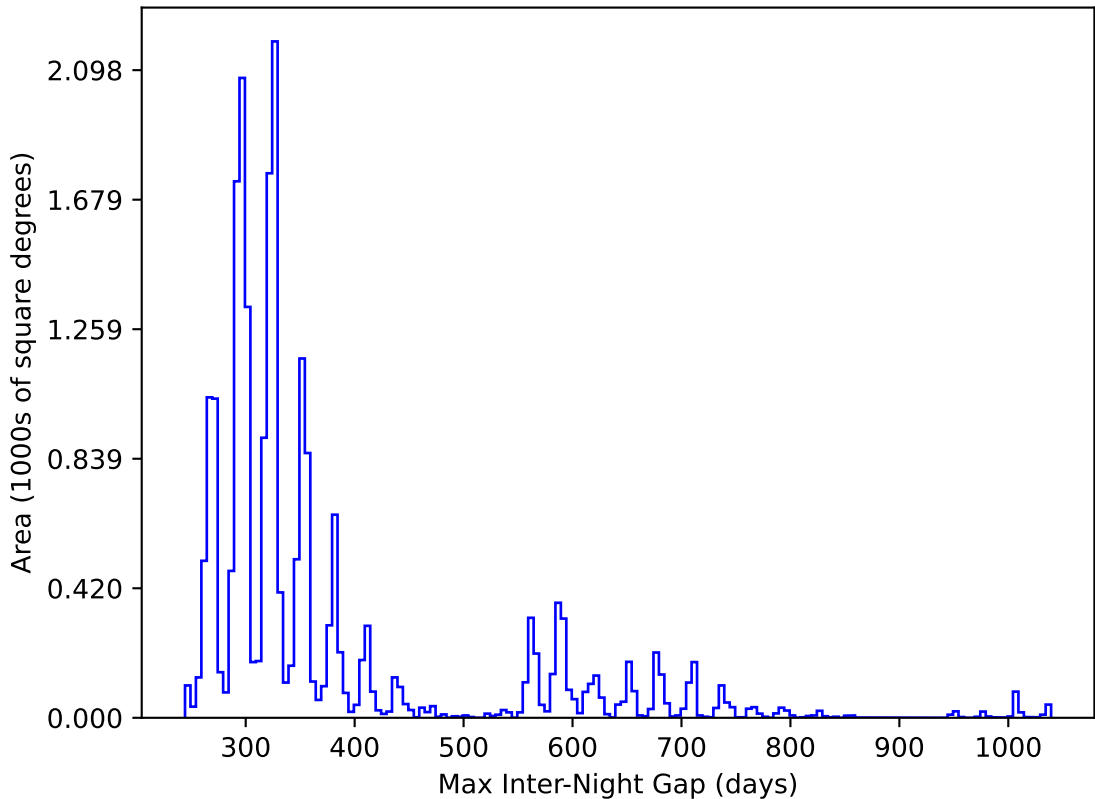
too_elab_r8_d2_griz_v3.4_10yrs All sky y band: Max Inter-Night Gap
