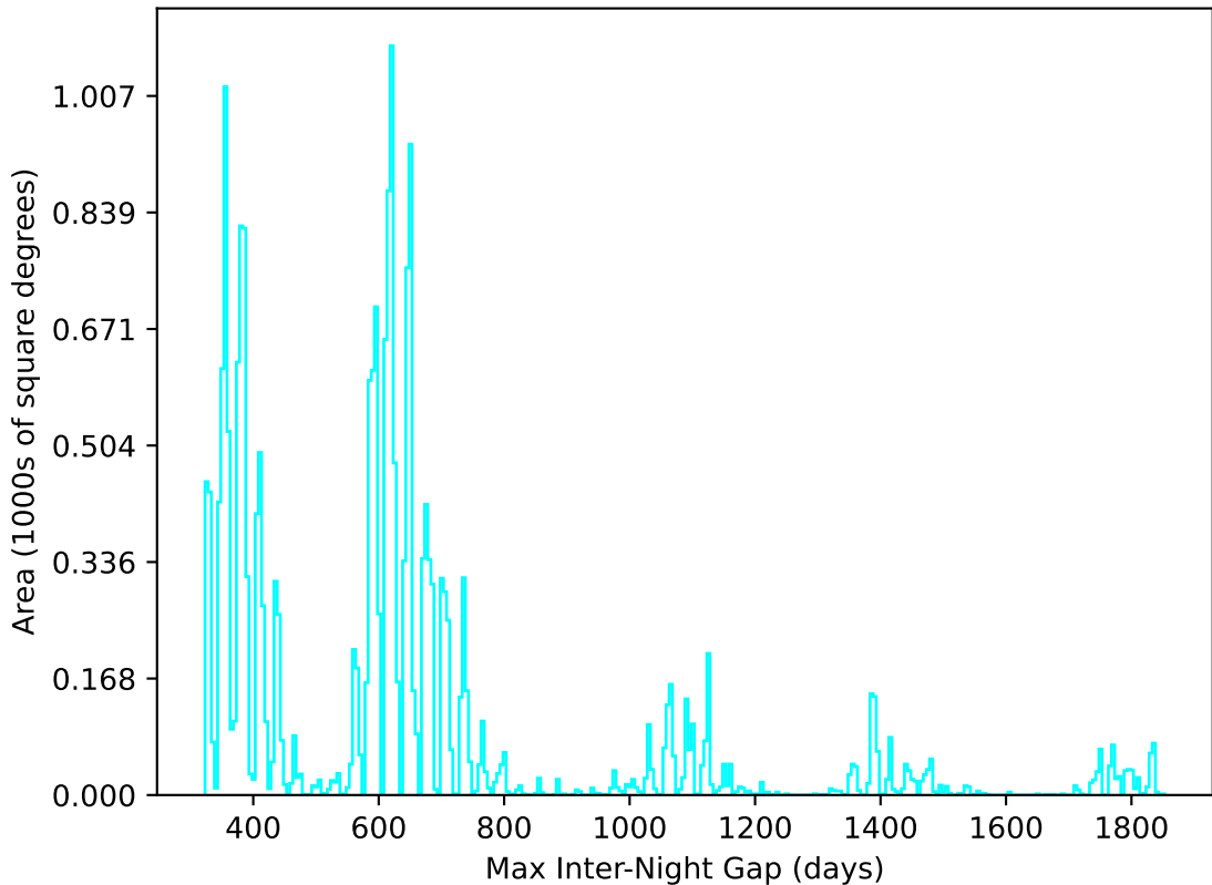
too_elab_r8_d2_griz_v3.4_10yrs All sky u band: Max Inter-Night Gap
