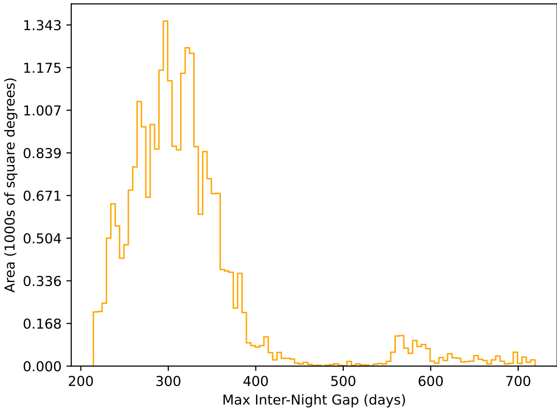
too_elab_r8_d2_griz_v3.4_10yrs All sky r band: Max Inter-Night Gap
