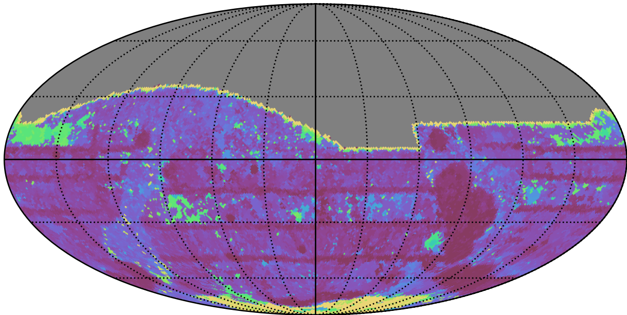
too_elab_r8_d2_griz_v3.4_10yrs All sky i band: Max Inter-Night Gap
