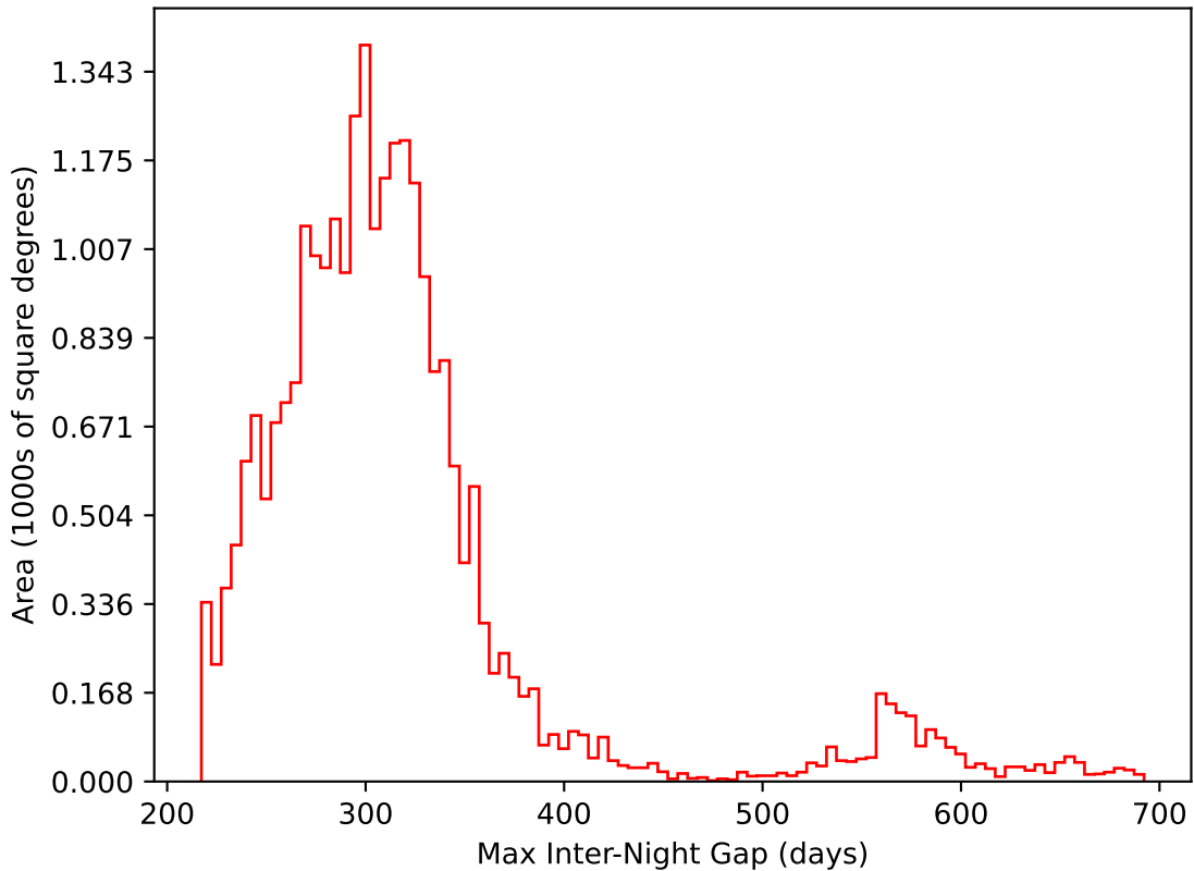
too_elab_r8_d2_griz_v3.4_10yrs All sky i band: Max Inter-Night Gap
