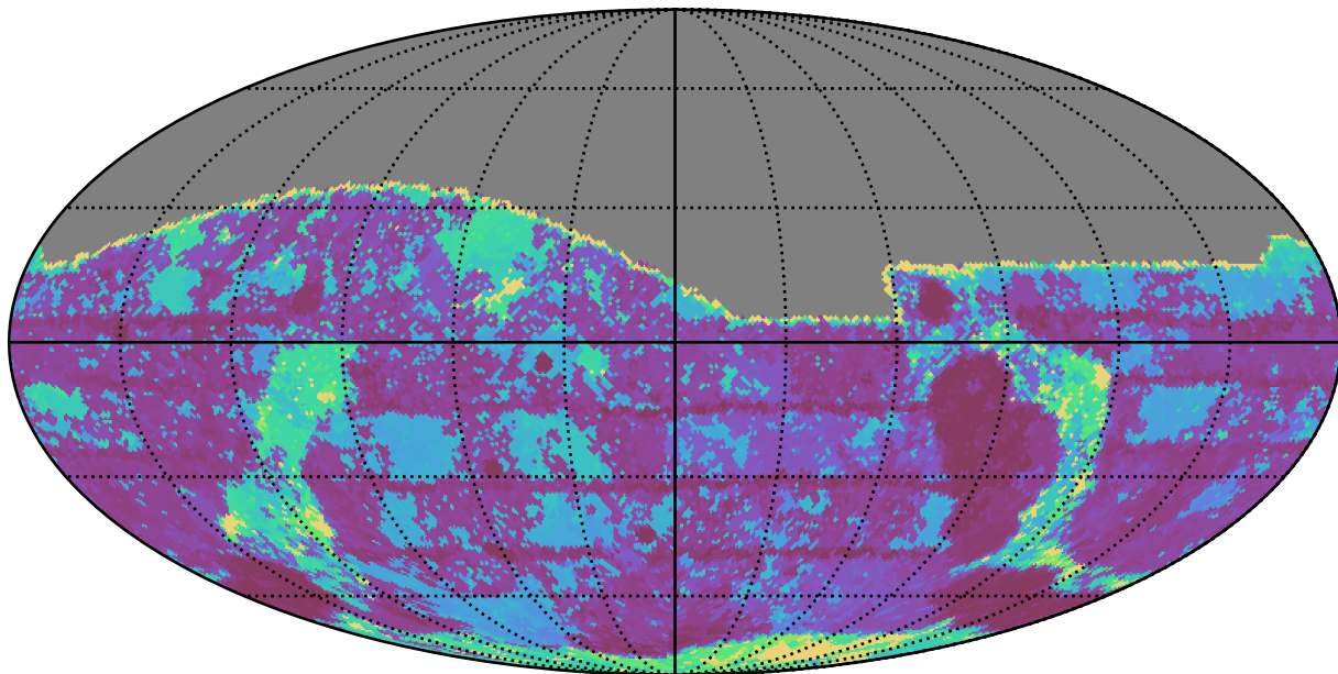
too_elab_r8_d2_griz_v3.4_10yrs All sky g band: Max Inter-Night Gap
