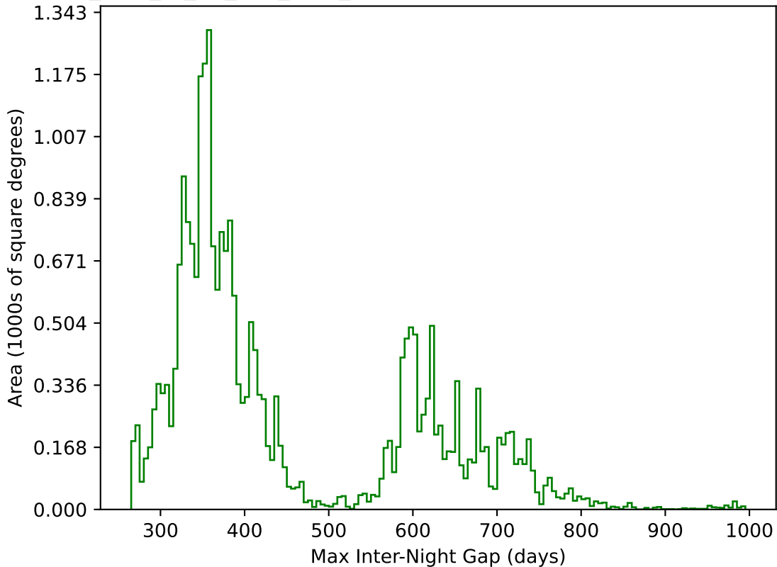
too_elab_r8_d2_griz_v3.4_10yrs All sky g band: Max Inter-Night Gap
