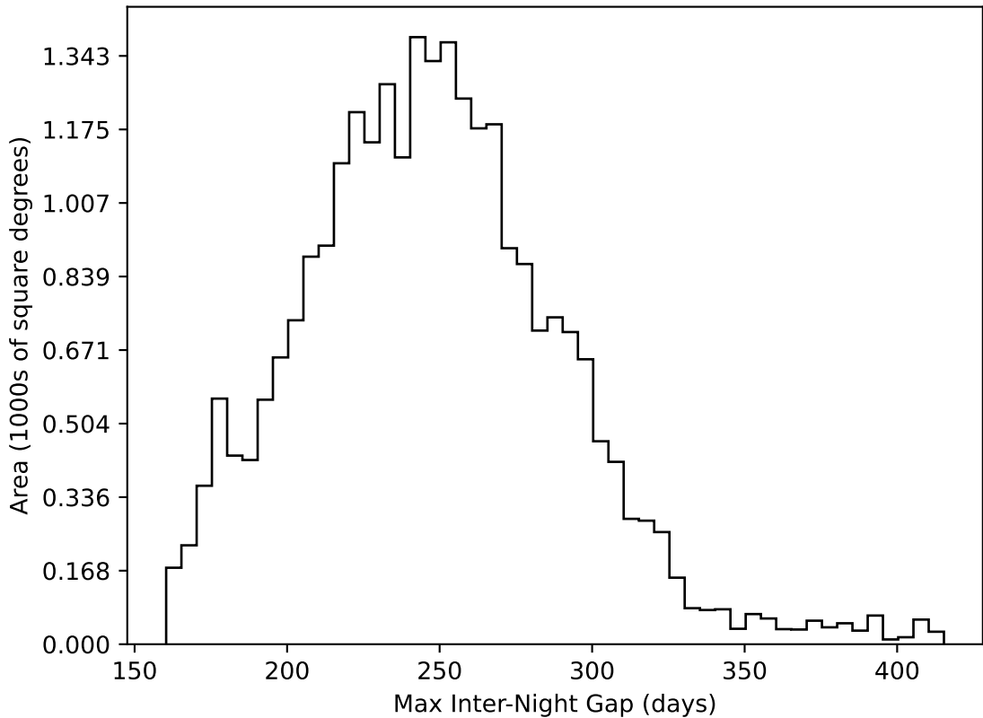
too_elab_r8_d2_griz_v3.4_10yrs All sky all bands: Max Inter-Night Gap
