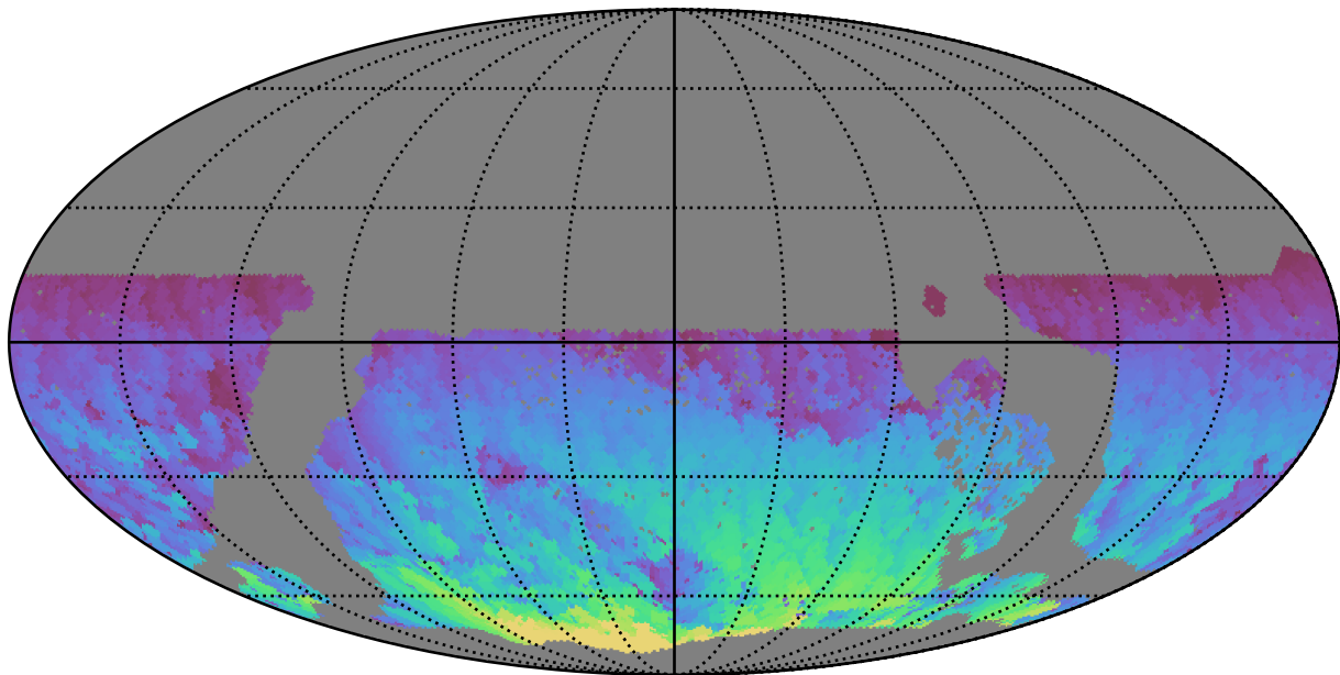
too_elab_r8_d2_griz_v3.4_10yrs WFD z band: Max HA
