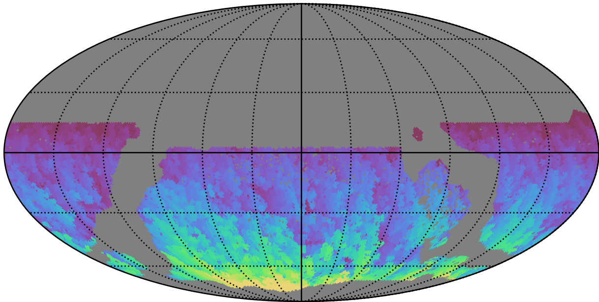
too_elab_r8_d2_griz_v3.4_10yrs WFD y band: Max HA
