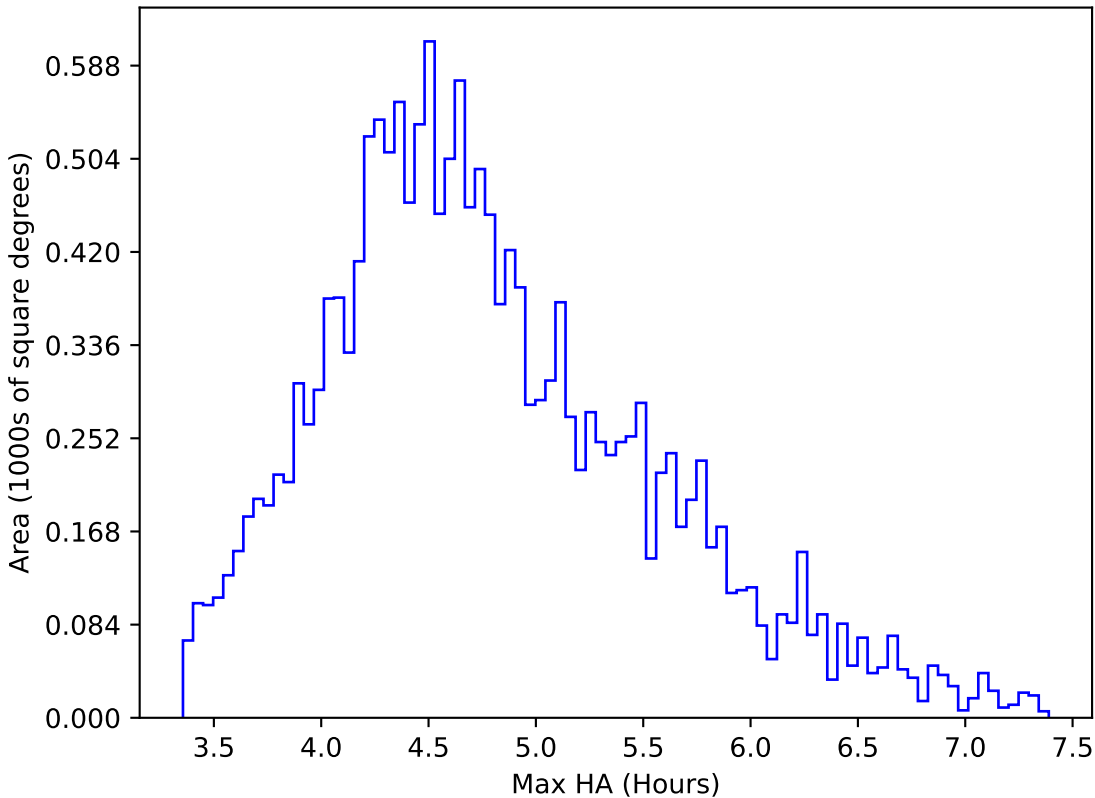
too_elab_r8_d2_griz_v3.4_10yrs WFD y band: Max HA
