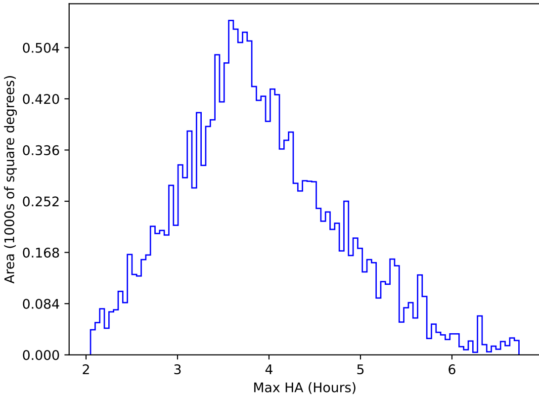
too_elab_r8_d2_griz_v3.4_10yrs WFD u band: Max HA
