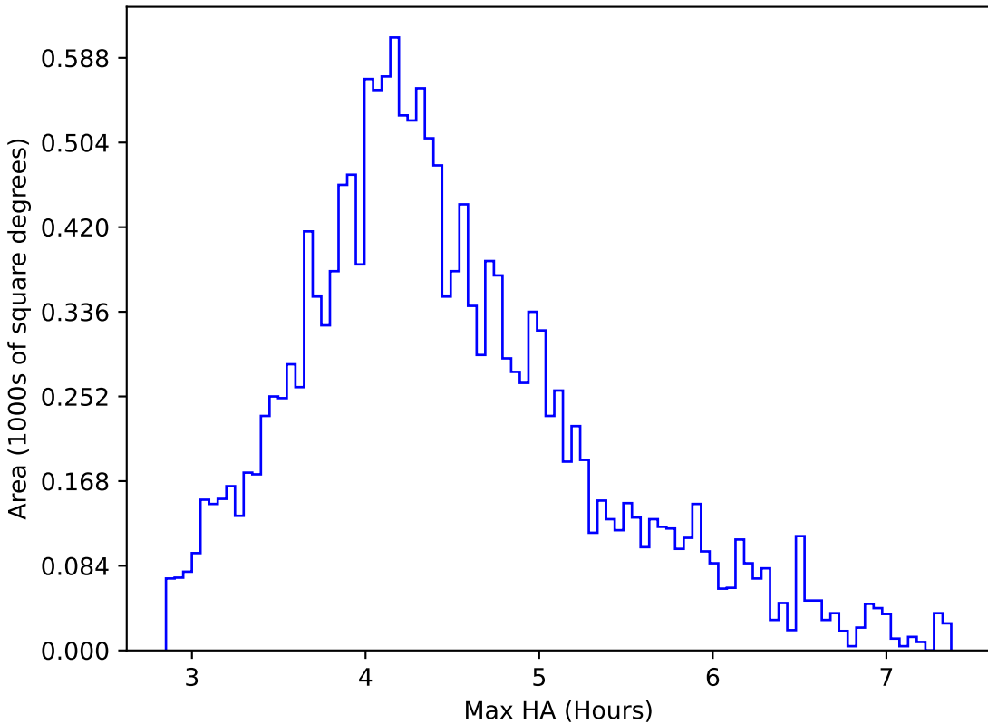
too_elab_r8_d2_griz_v3.4_10yrs WFD r band: Max HA
