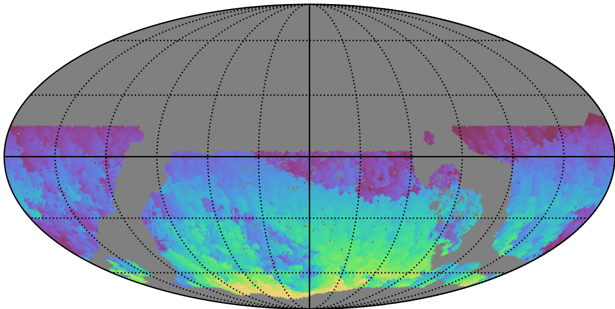
too_elab_r8_d2_griz_v3.4_10yrs WFD i band: Max HA
