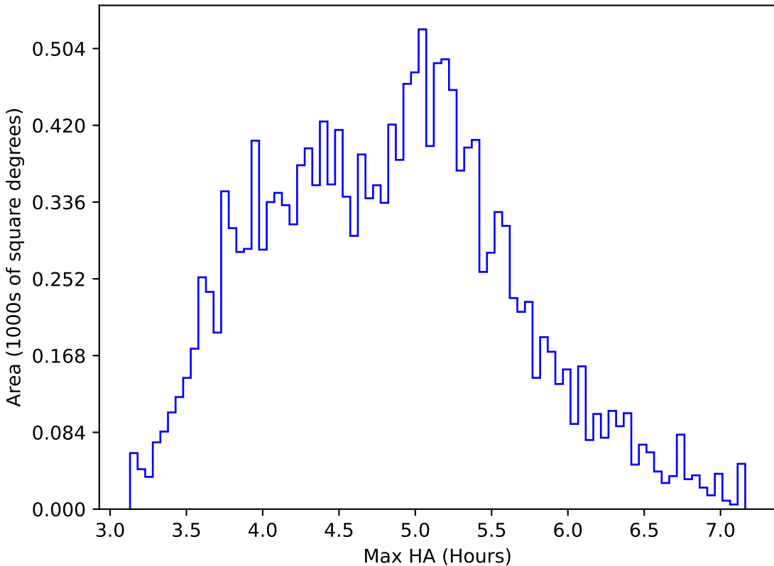
too_elab_r8_d2_griz_v3.4_10yrs WFD i band: Max HA
