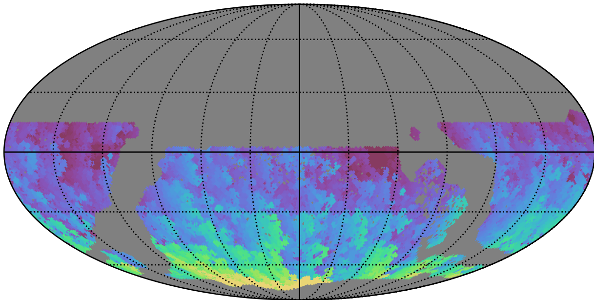
too_elab_r8_d2_griz_v3.4_10yrs WFD g band: Max HA
