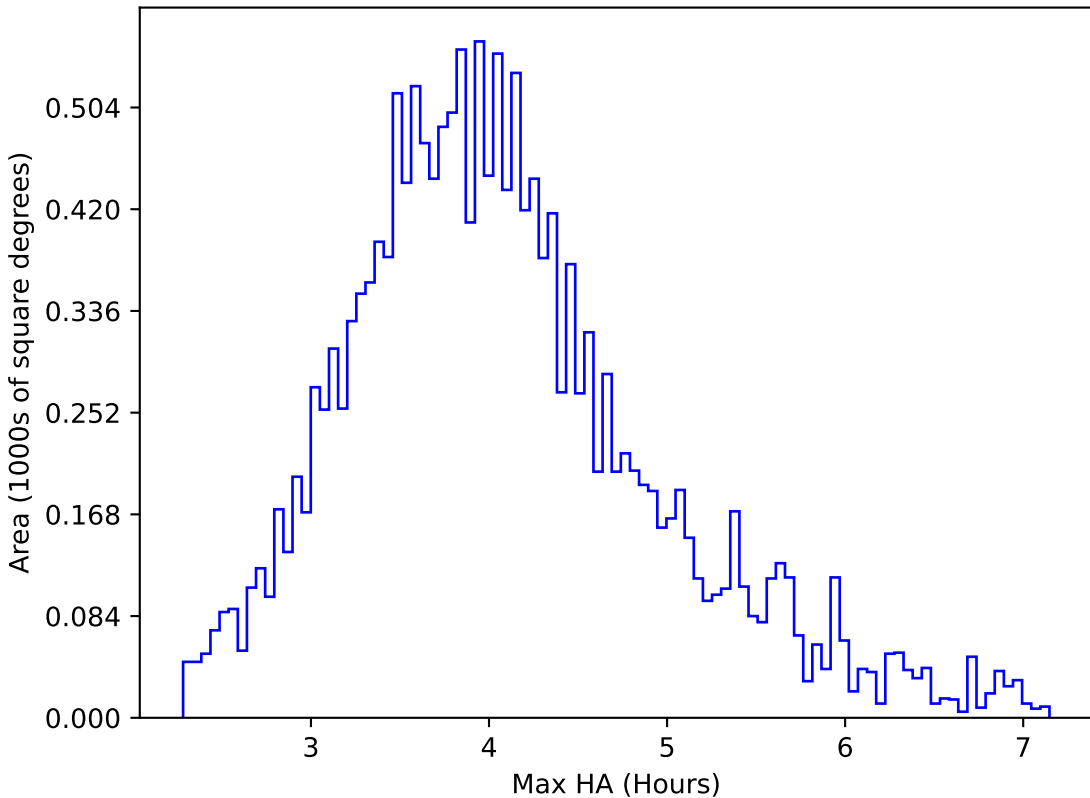
too_elab_r8_d2_griz_v3.4_10yrs WFD g band: Max HA
