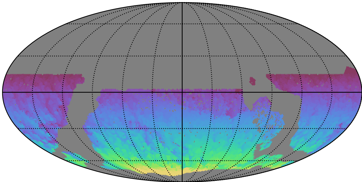
too_elab_r8_d2_griz_v3.4_10yrs WFD all bands: Max HA
