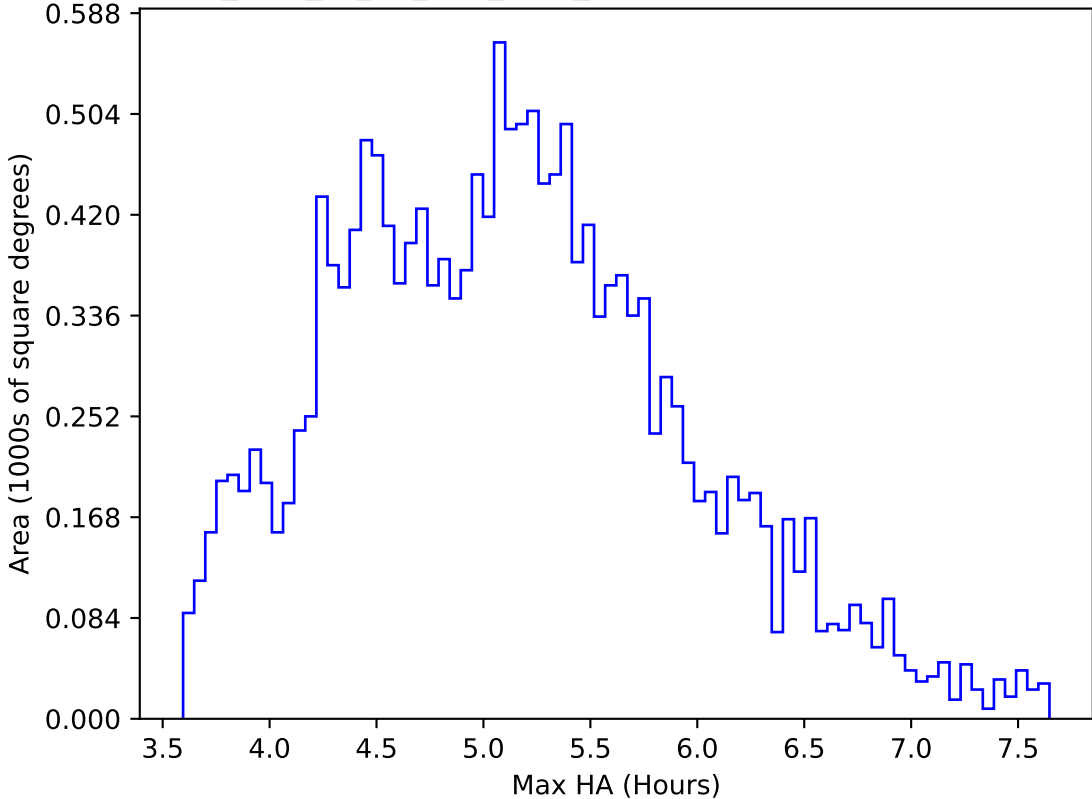
too_elab_r8_d2_griz_v3.4_10yrs WFD all bands: Max HA
