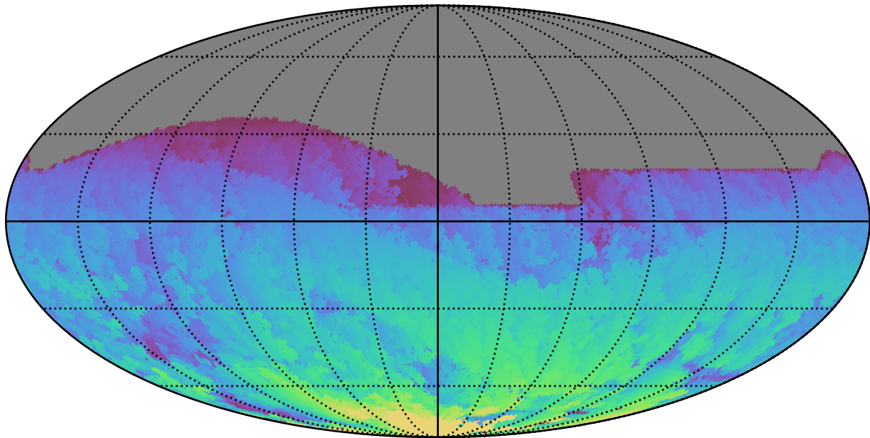
too_elab_r8_d2_griz_v3.4_10yrs All sky z band: Max HA
