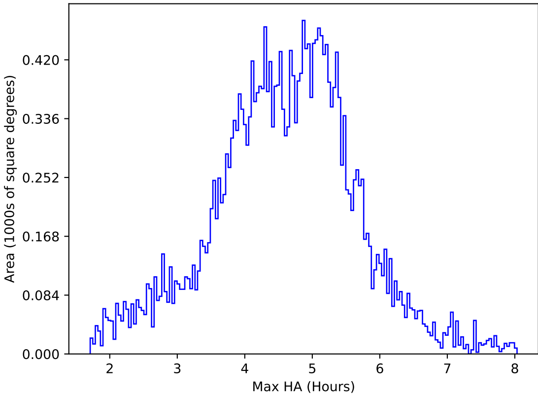
too_elab_r8_d2_griz_v3.4_10yrs All sky z band: Max HA
