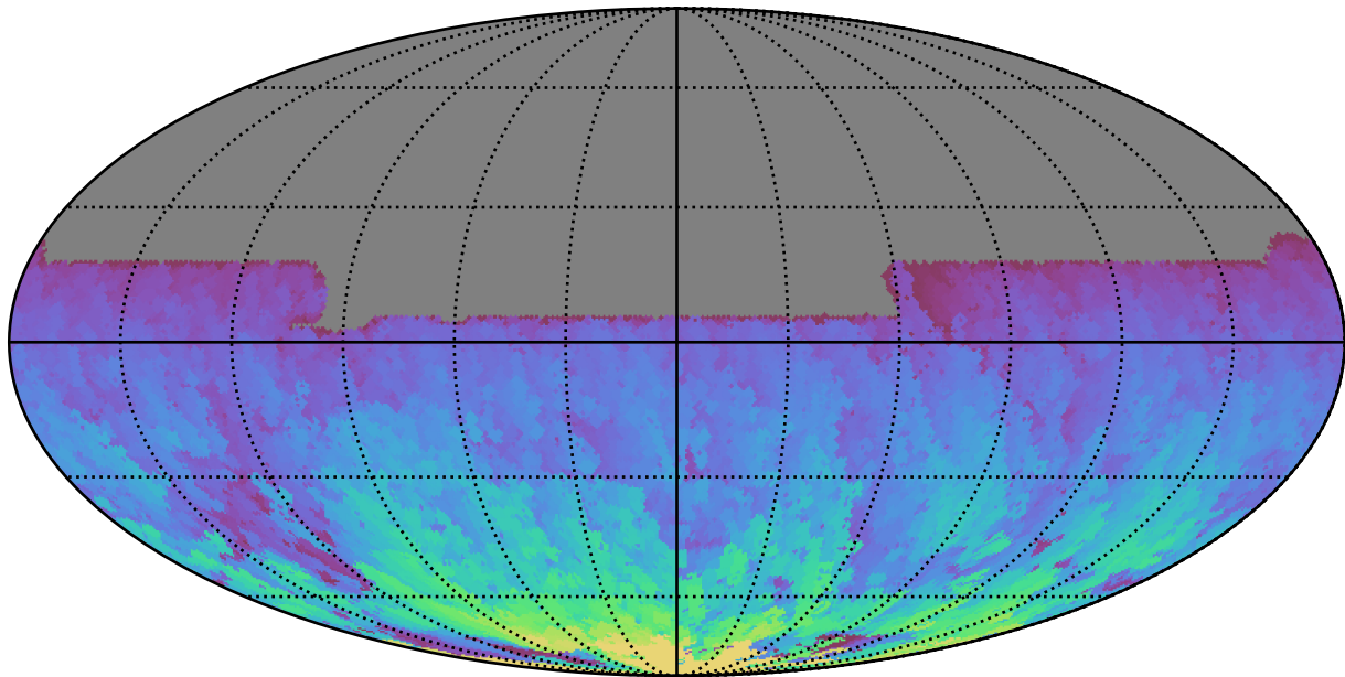
too_elab_r8_d2_griz_v3.4_10yrs All sky y band: Max HA
