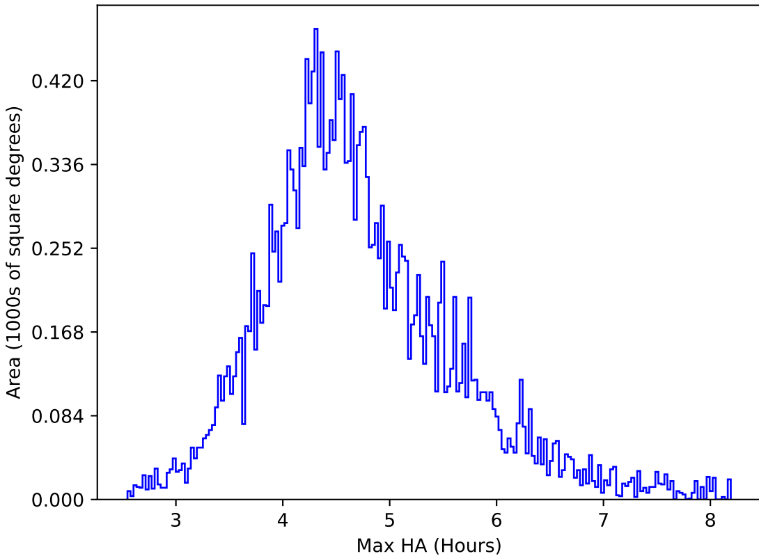
too_elab_r8_d2_griz_v3.4_10yrs All sky y band: Max HA
