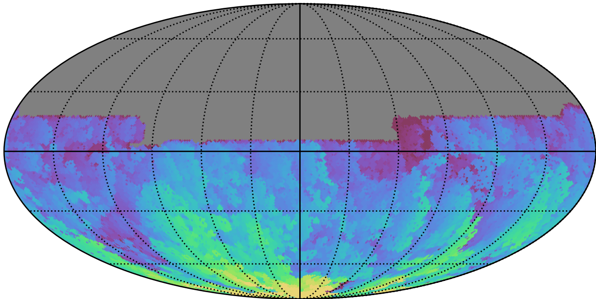
too_elab_r8_d2_griz_v3.4_10yrs All sky u band: Max HA
