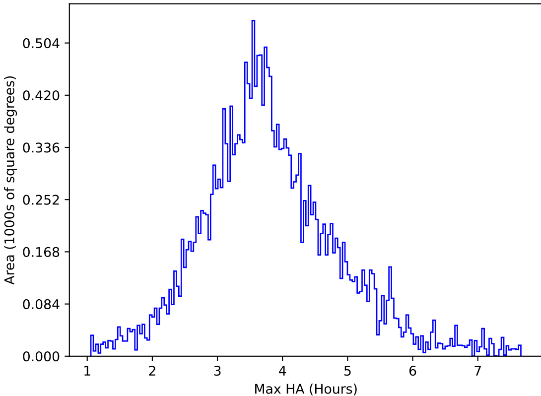
too_elab_r8_d2_griz_v3.4_10yrs All sky u band: Max HA
