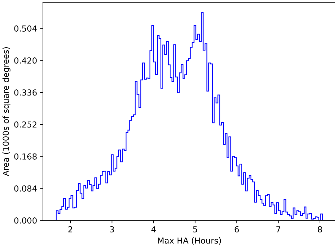
too_elab_r8_d2_griz_v3.4_10yrs All sky i band: Max HA
