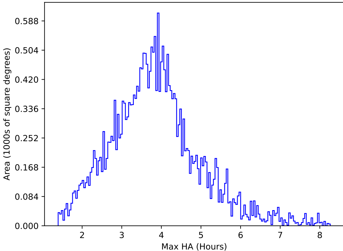
too_elab_r8_d2_griz_v3.4_10yrs All sky g band: Max HA
