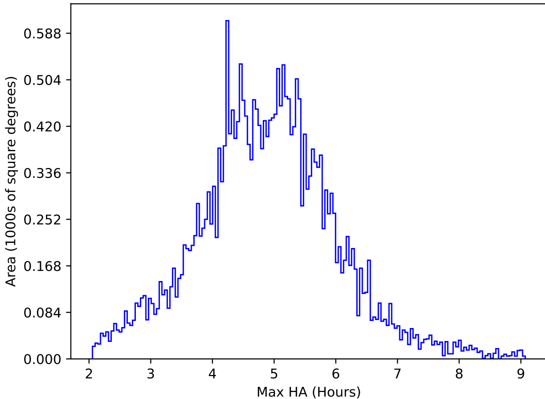
too_elab_r8_d2_griz_v3.4_10yrs All sky all bands: Max HA
