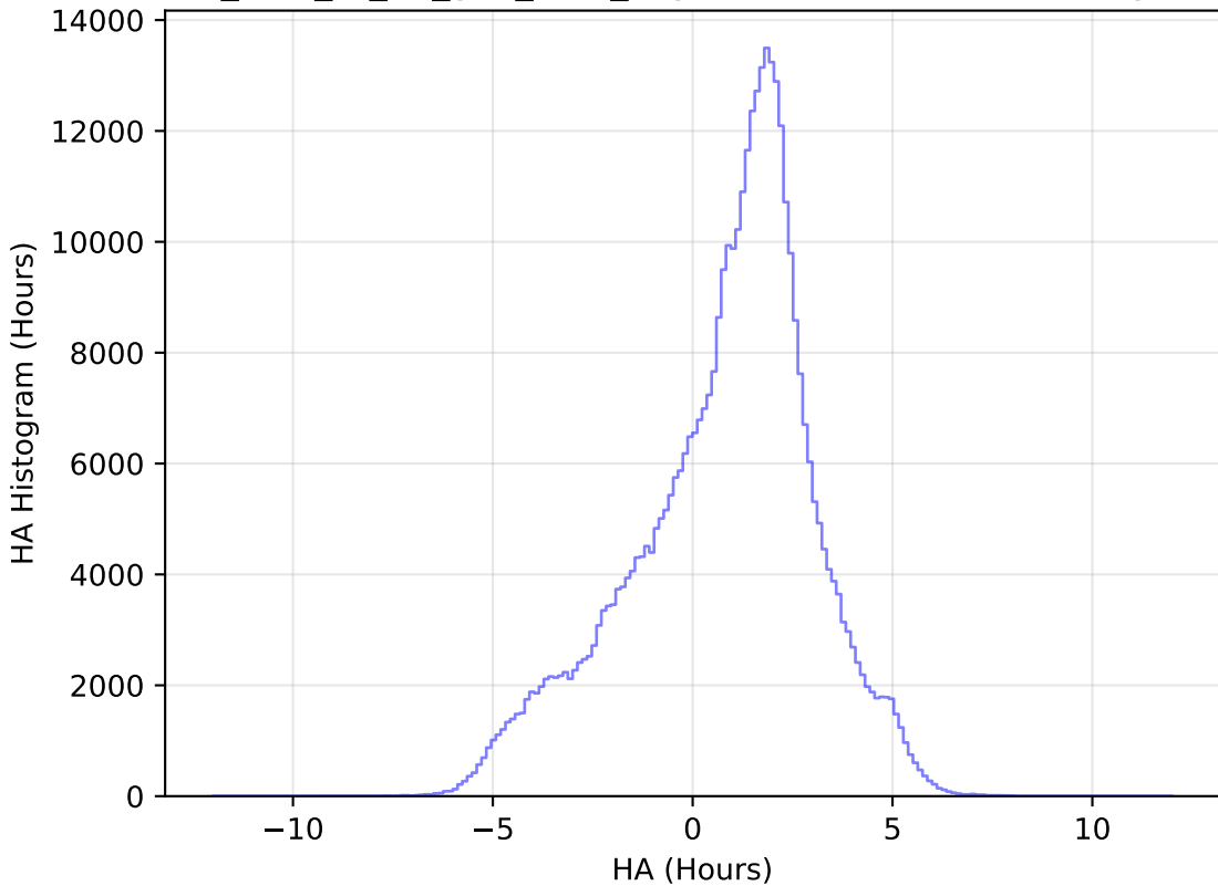
too_elab_r8_d2_griz_v3.4_10yrs WFD z band: HA Histogram
